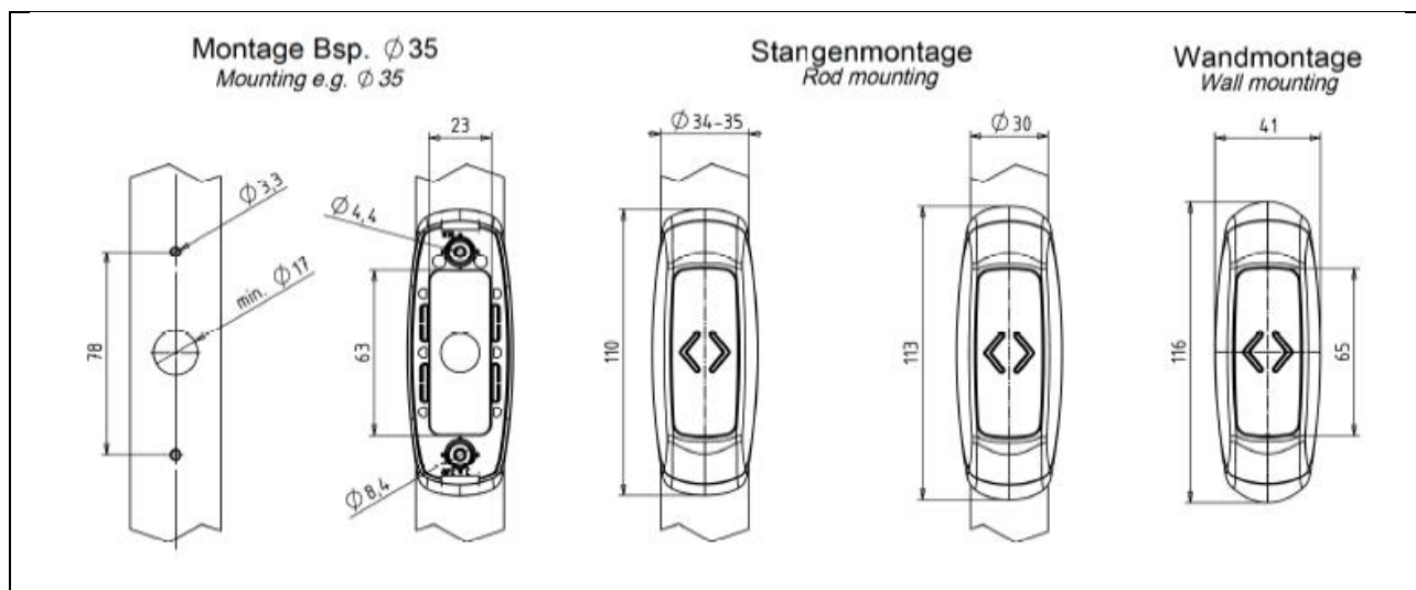
Abbildung 1: SENSORtaster HWT2 series – Quelle: Captron
