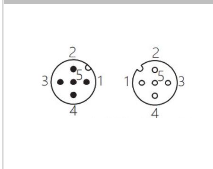
Stecker M12, 5-polig Connector M12, 5-pole
